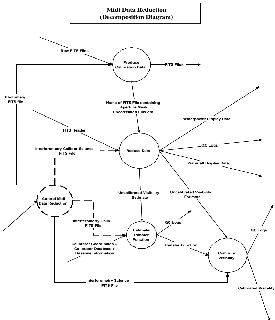
Figure D.1: MIDI Pipeline High-Level Functional Diagram
