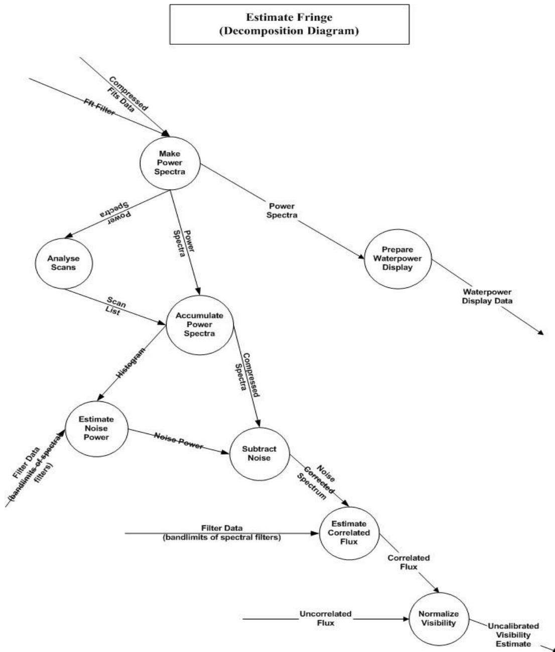
Figure D.2: Functional Diagram: MIDI Visibility Estimates
